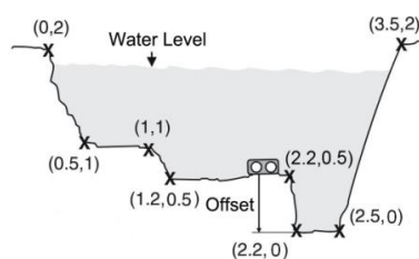
Irregular-shaped channel
