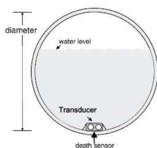
Partially pipe
