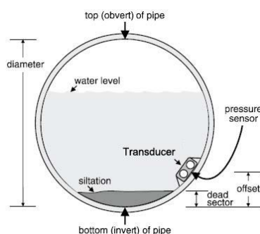
Pipe with siltation on bottom
