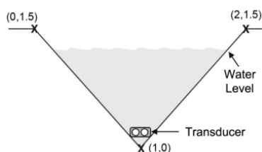
Triangle Channel
